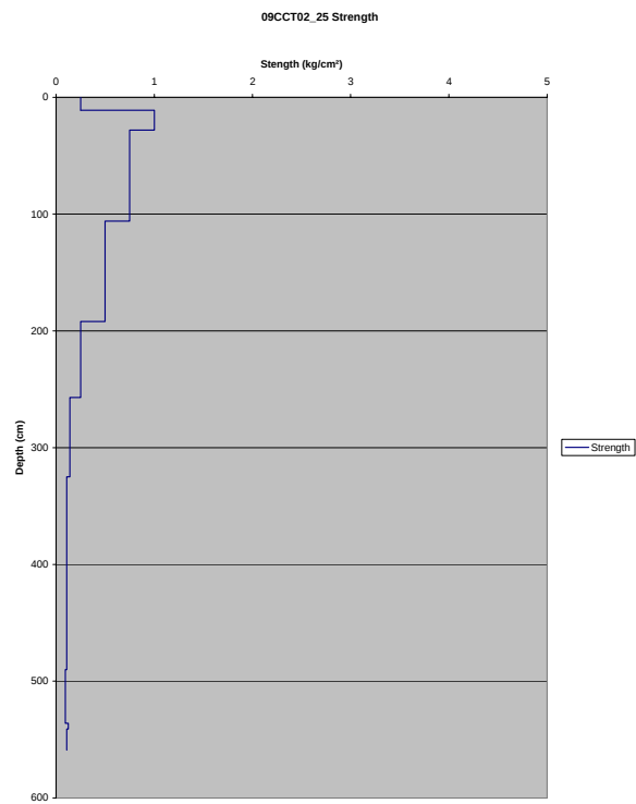
09CCT02_25 Strength Graph
