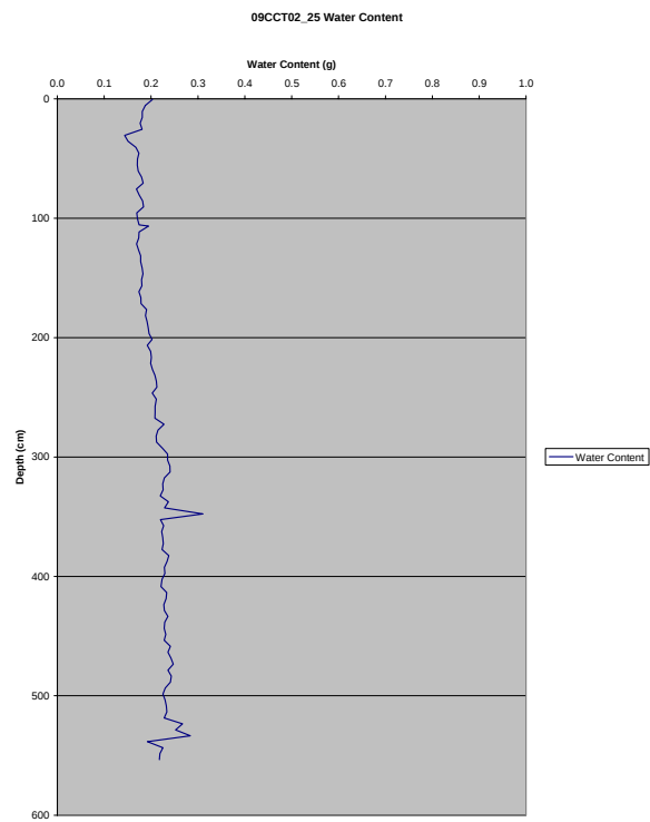
09CCT02_25 Water Content Graph
