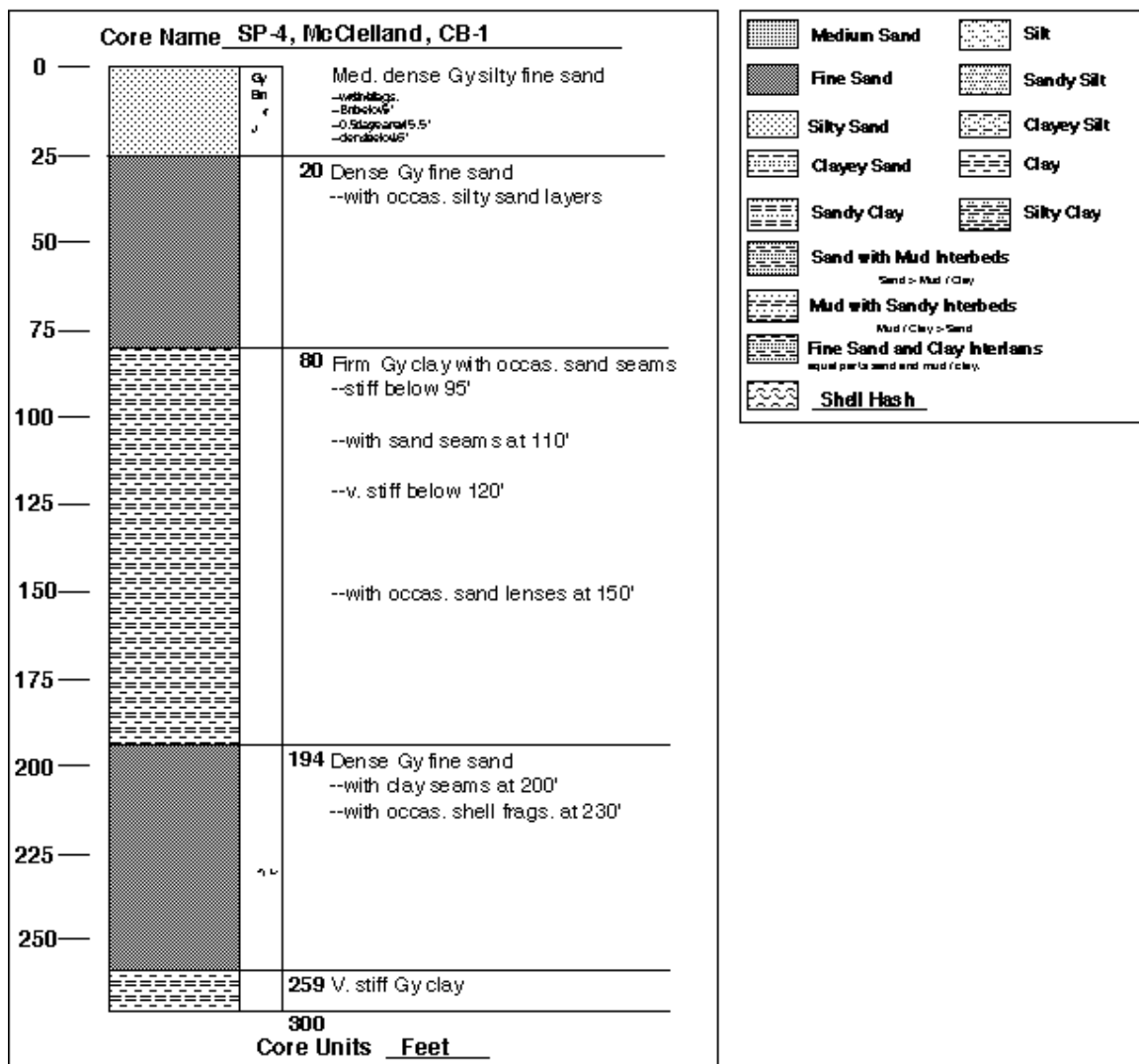
Figure 8. – Boring description SP-4. See Figure 4 for location.
