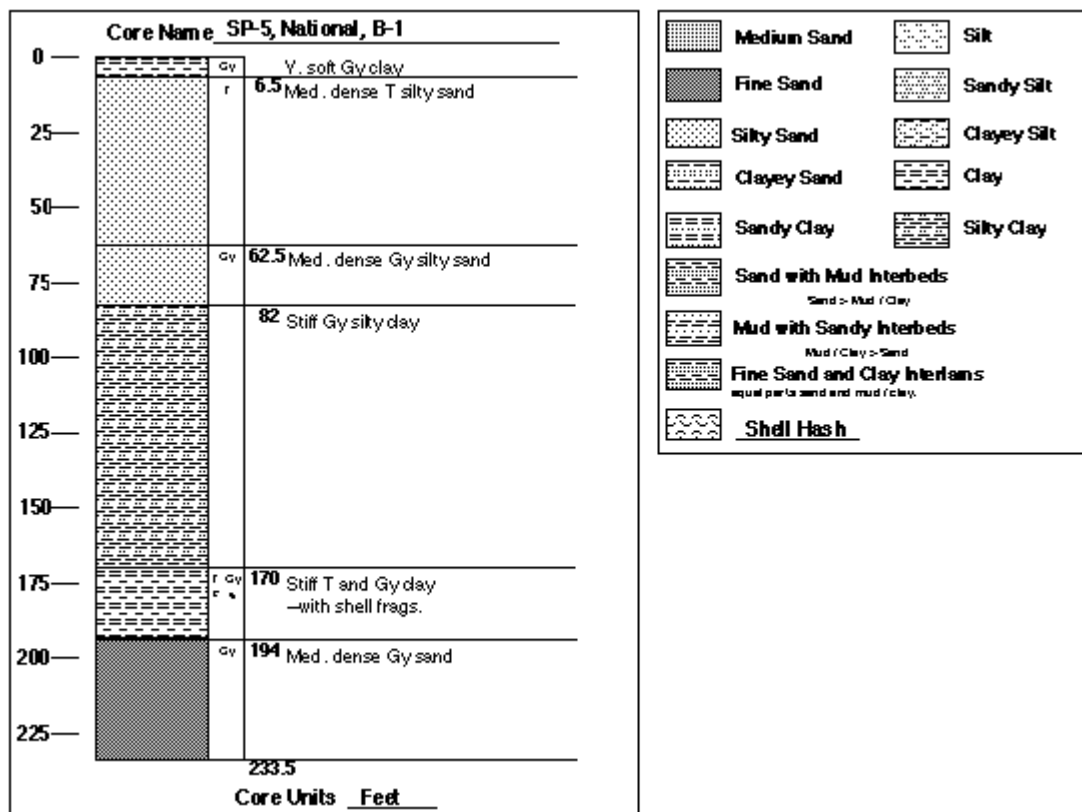
Figure 9. – Boring description SP-5. See Figure 4 for location.
