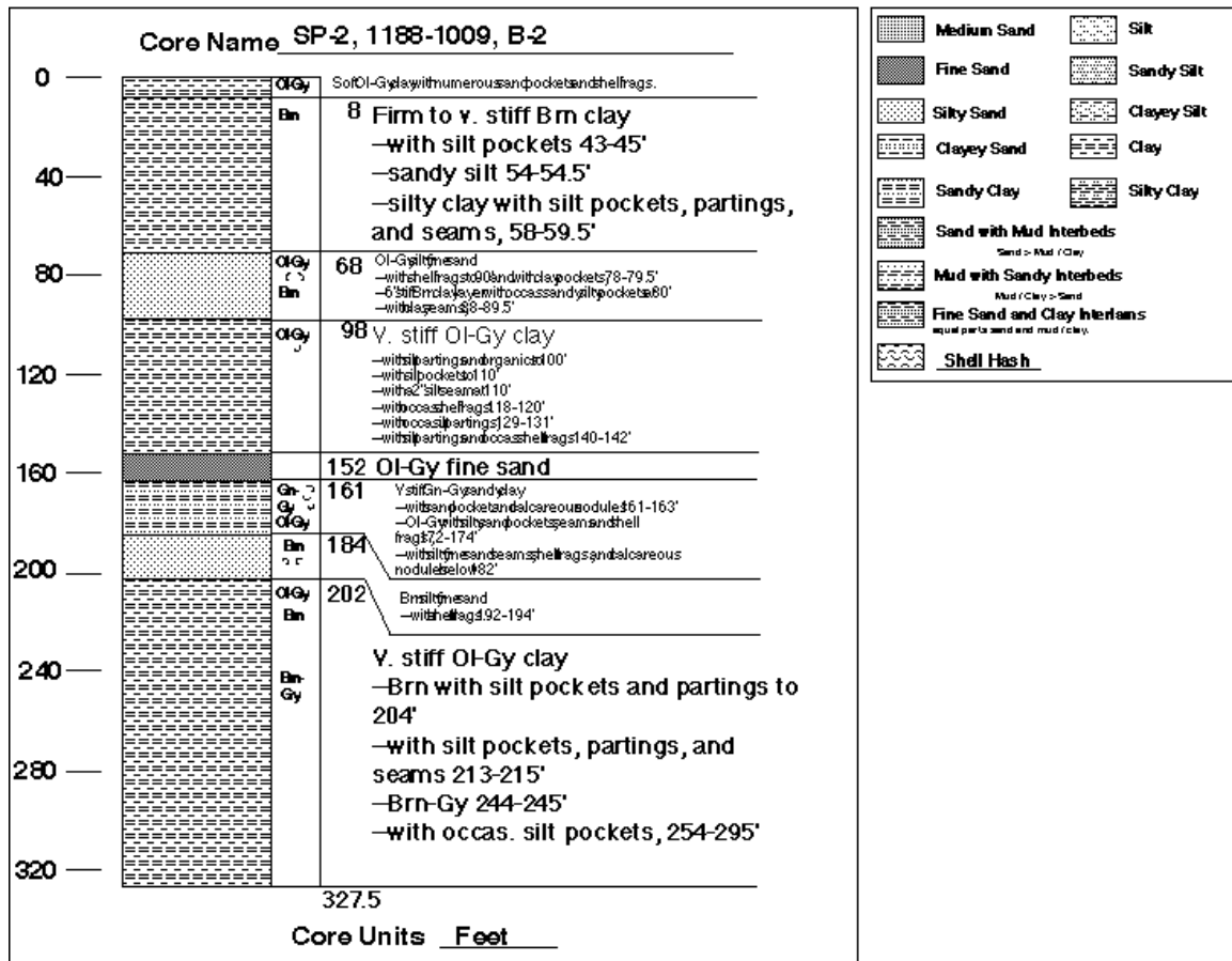
Figure 5. – Boring description SP-2. See Figure 4 for location.
