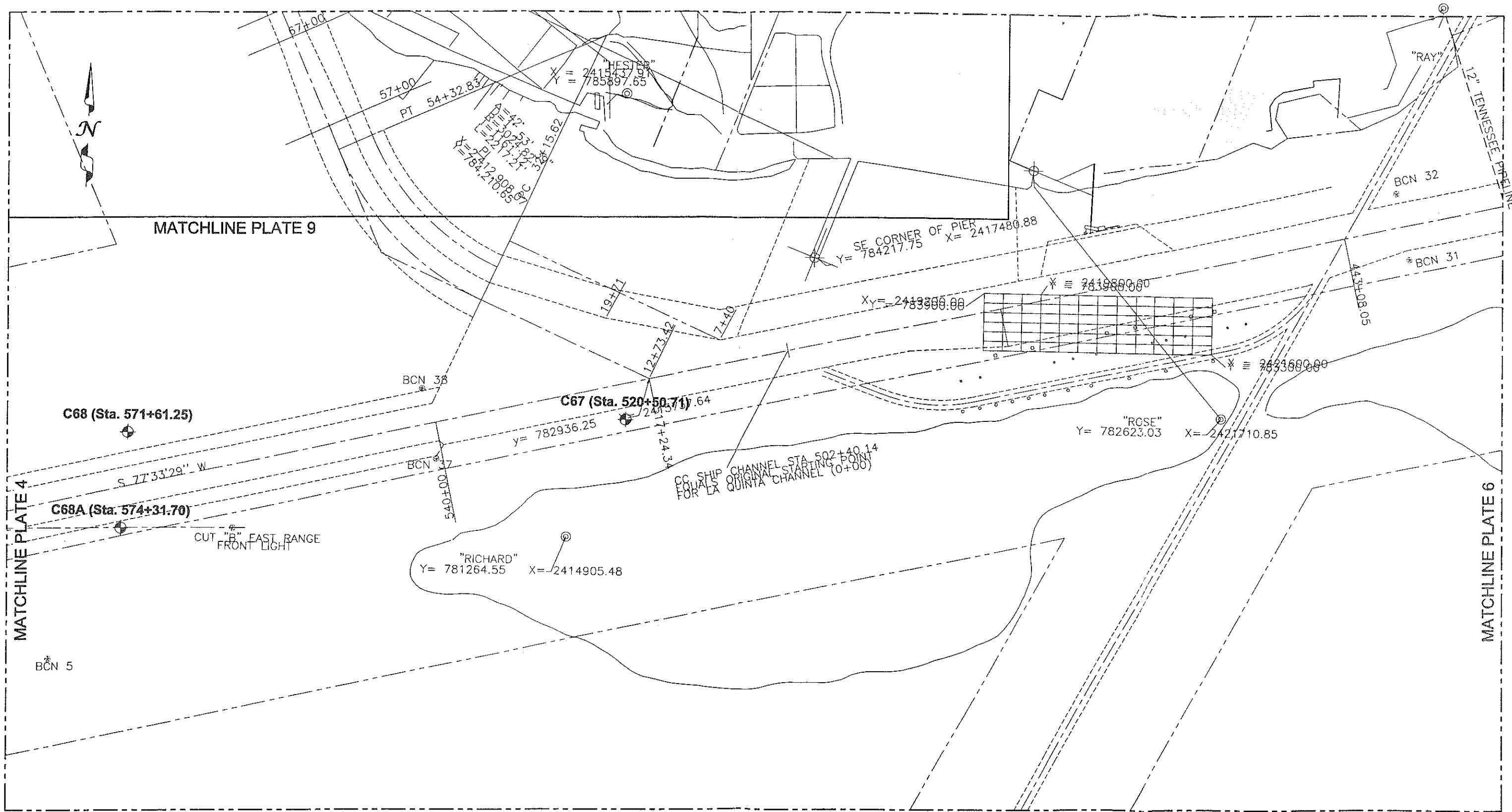
PLAN OF BORINGS
